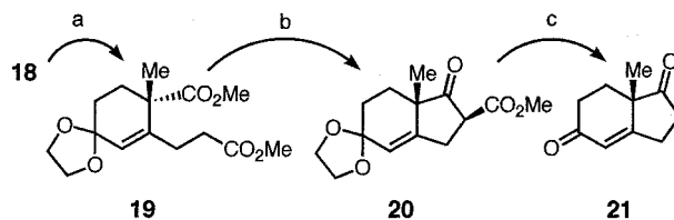
Scheme 8. Chemical derivatization of Hagemann's ester 18 into bicyclic dione 21 : reagents and conditions: (a) TMSOCH 2 CH 2 .OTMS, TMSOTf, 20 h, -78 °C; (b) MeONa, benzene at reflux, 2 h; (c) MgCl 2 hexahydrate, DMSO, 130 °C
